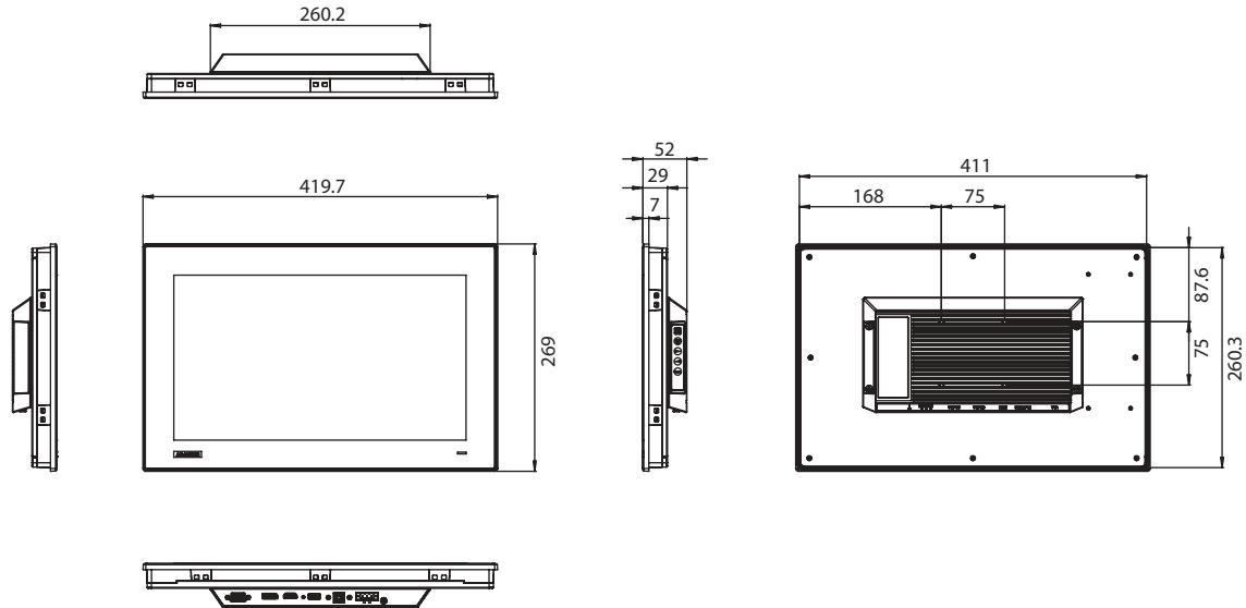
Panel Cutout Dimensions: FPM-715W: 412.4 x 261.7 mm (16.24 x 10.30 in)
