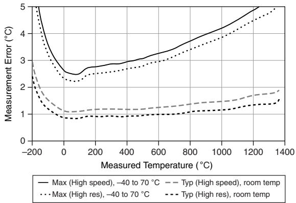
Figure 3. Thermocouple Type K Errors
