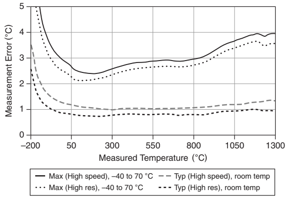
Figure 3. Thermocouple Type K Errors
