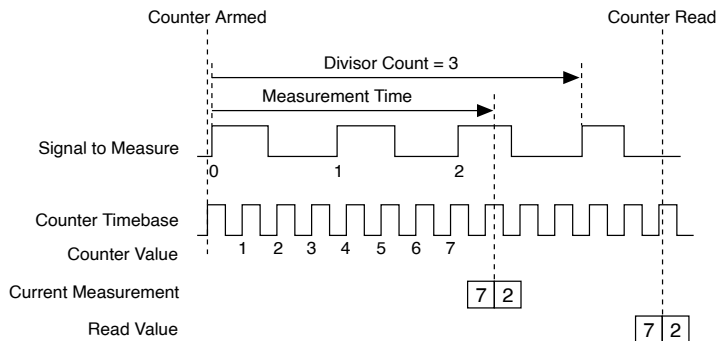
Figure 10. Measurement Time completes before Divisor
