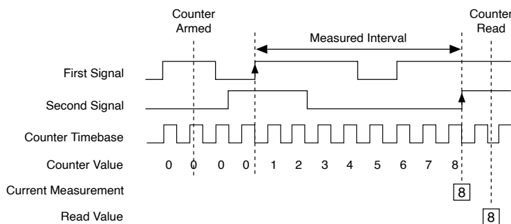
Figure 12. Two-Edge Separation
