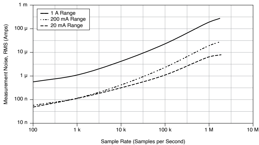
Figure 5. PXIe-4082 Current Waveform Noise, Typical
